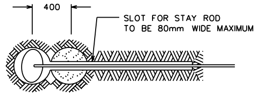
DOUBLE AUGURED HOLE
