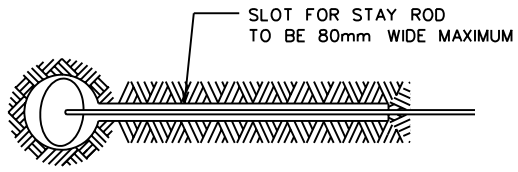
SINGLE AUGURED HOLE
